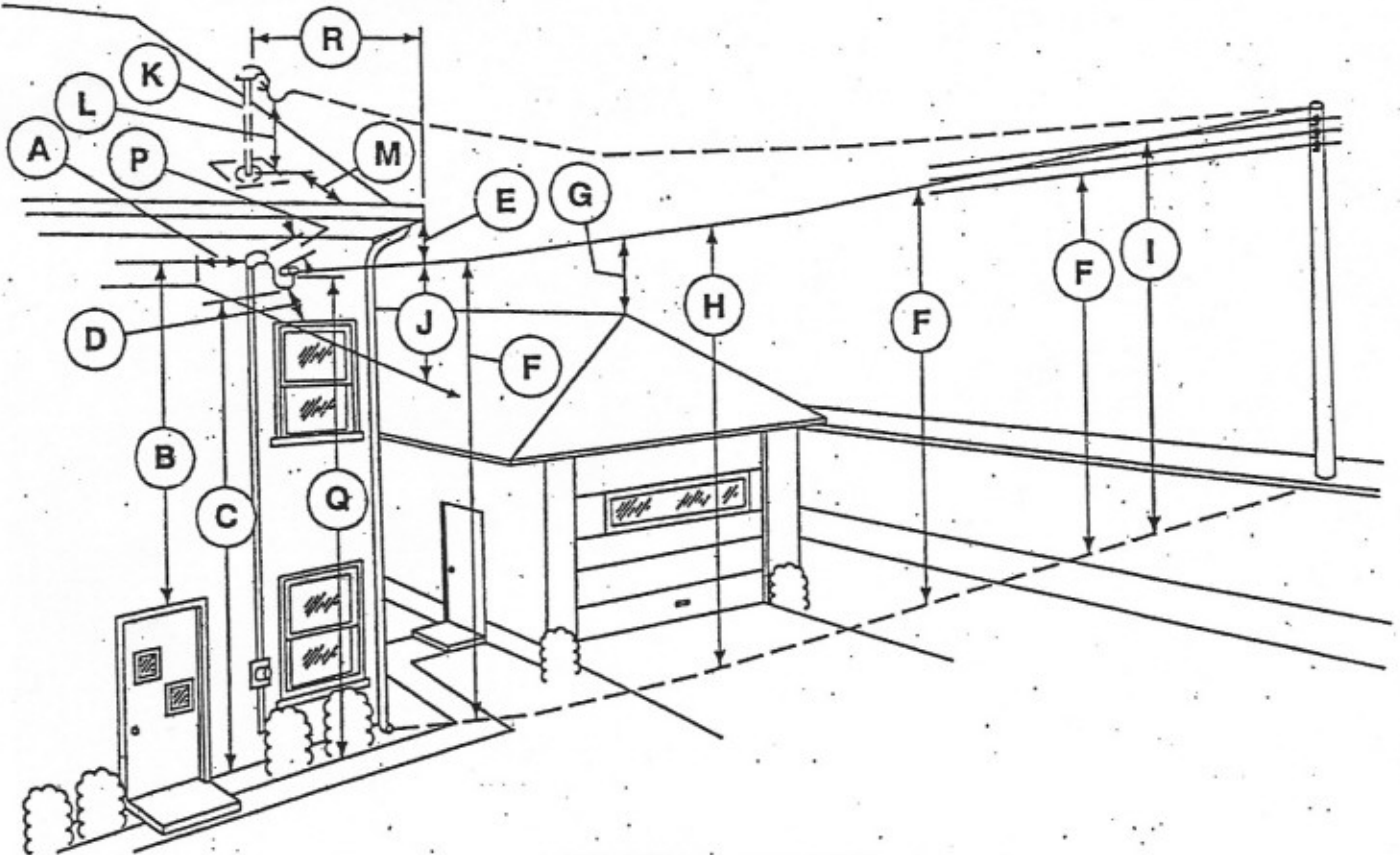
MINIMUM CLEARANCE
